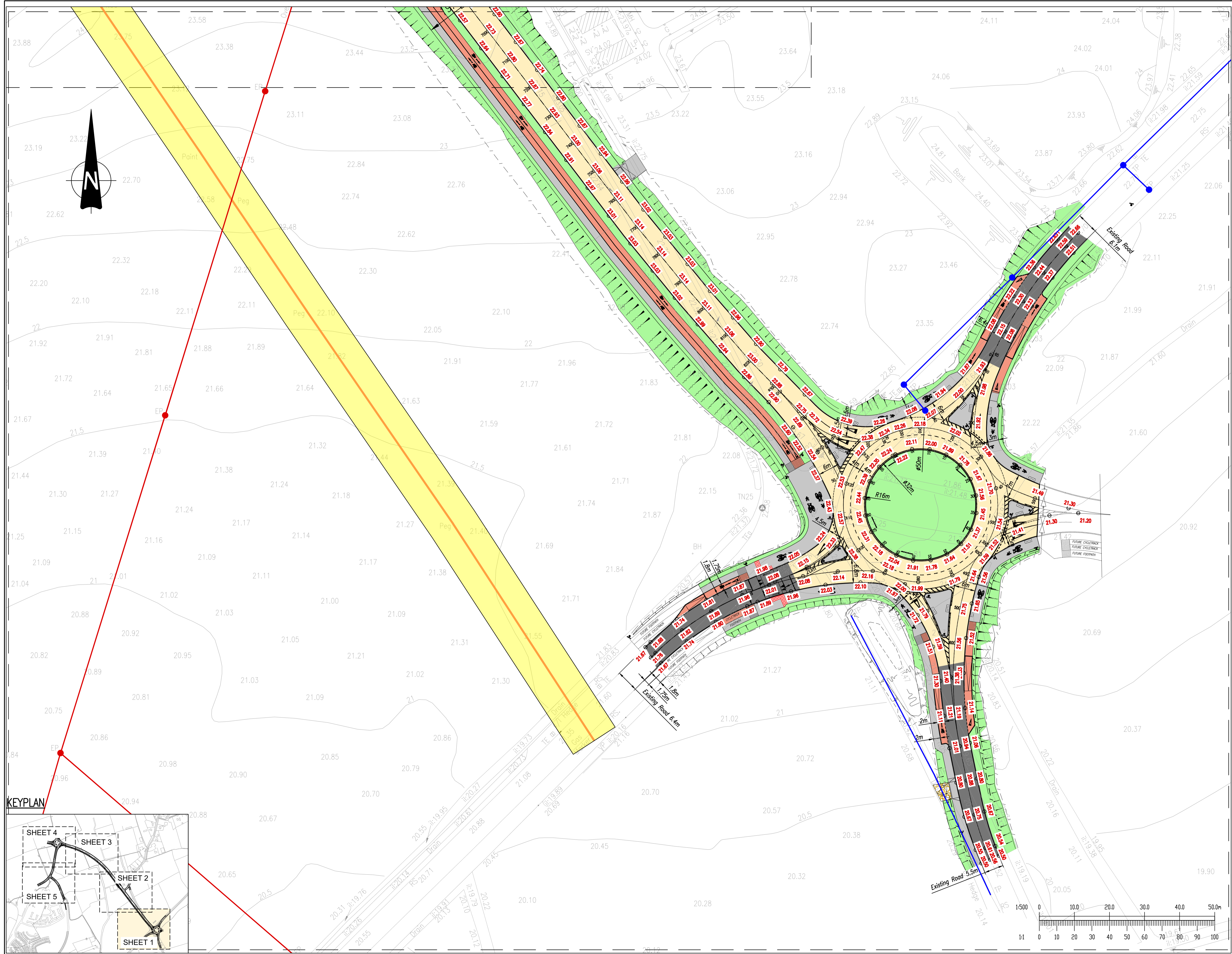
PLAN VIEW - PROPOSED ROADS LAYOUT AND LEVELS - SHEET 1 OF 5 SCALE 1:500 @A1
